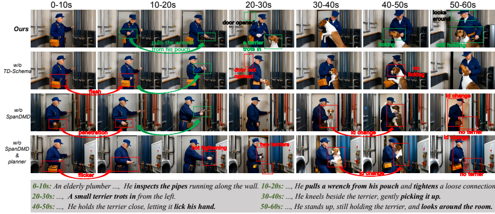
Figure 4: Ablation on a six-prompt stream (prompts at the bottom). Green marks the intended progression; red marks failures such as flicker, interpenetration, duplicated or missing terriers, and identity changes.
