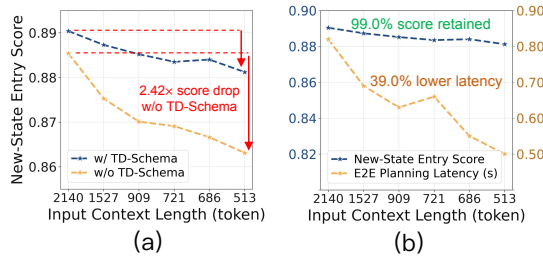
Figure 5: Planning quality and latency as the planner’s input context shrinks, with and without TD-Schema.
