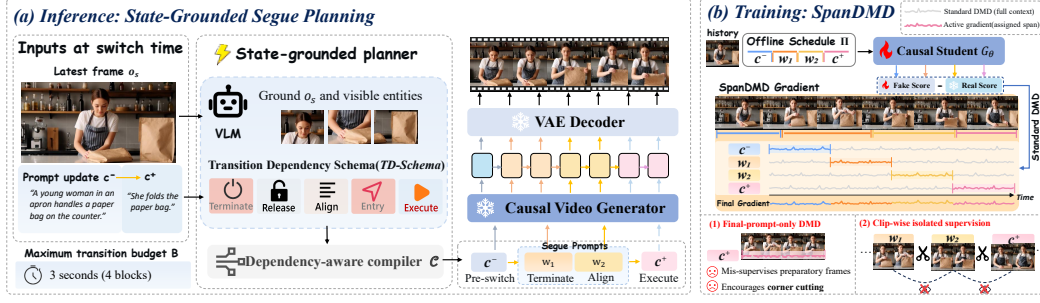
Figure 2: Overview of SEGUE. At a switch, the planner reads the latest generated frame, the user prompts c^- and c^+ , and the transition budget B , and compiles a dependency-aware segue schedule under the TD-Schema leading to c^+ ; the causal generator executes this schedule block by block. During training, SPANDMD evaluates the complete rollout under each active prompt, including c^- and c^+ , while retaining each prompt’s DMD residual only on its assigned temporal span. The bottom-right illustrates two alternative supervision choices motivating SPANDMD.
