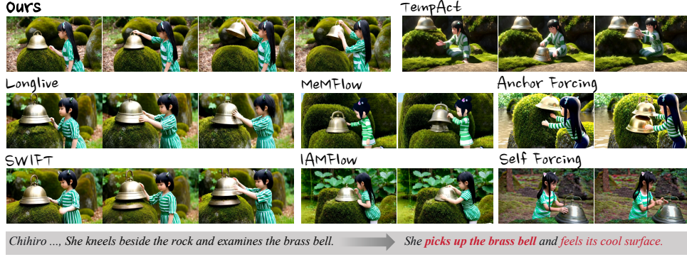
Figure 3: Comparison at the switch from “She kneels beside the rock and examines the brass bell” to “She picks up the brass bell and feels its cool surface.” SEGUE grasps and lifts the existing bell; TempAct and Anchor Forcing duplicate it, and several baselines never reach a lifted state.
