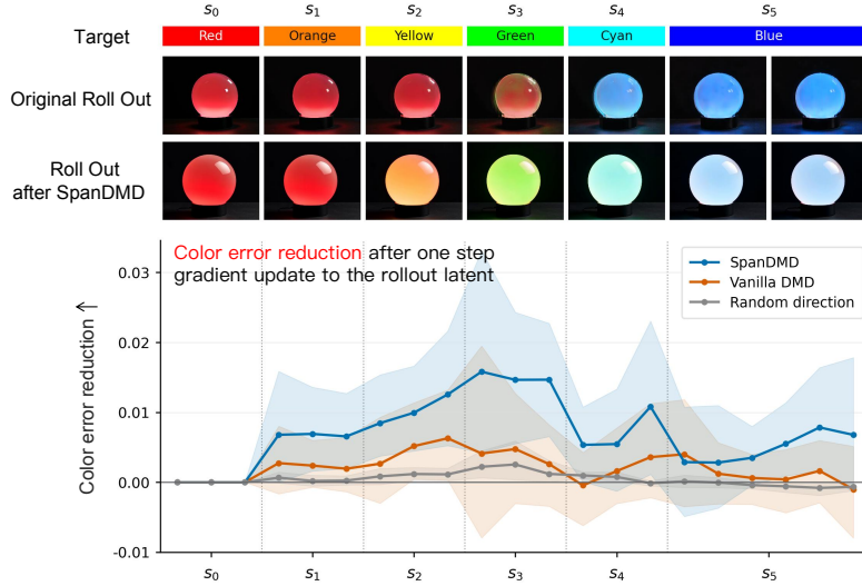
Figure 9: Color-sequence evaluation. Top: Qualitative examples of generator outputs before and after SpanDMD training, shown alongside the target color of each span. Bottom: A latent-update diagnostic measuring mean color-error reduction after one equal-magnitude update over 200 videos, starting from shared initial latents with all model parameters frozen. Shaded bands show pointwise 95% paired hierarchical bootstrap confidence intervals.
