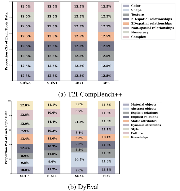
Fig. 6. Comparison of static (T2I-CompBench++) and dynamic (DyEval) test input distributions across models.
