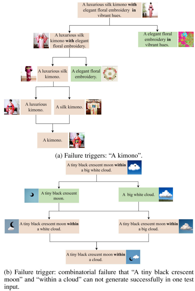
Fig. 13. Two examples of dynamic failure location. Bold are the relation nodes in their scene graph form. green means test input passes, and brown means test input fails.
