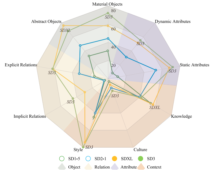
Fig. 7. Average test pass rate APR of SD1-5, SD2-1, SDXL, and SD3 models in nine dimensions. Dimensions of the same base color indicate belonging to the same category. The overall trend of image generation capabilities is SD3 \geq SDXL > SD2-1 > SD1-5 ; culture and implicit relations are the weakest part of all models. We label the best-performing models in different dimensions with the its name.
