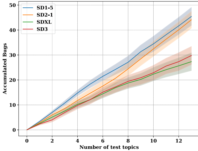
Fig. 4. Average number of bugs accumulated within an initial topic throughout thirteen test nodes ( 1 + 1 \times 3 + 3 \times 3 ) during the testing process of DyEval of SD1-5, SD2-1, SDXL, SD3. The standard error is over nine initial topics. The index of the test node of the test tree is obtained according to the breadth-first search. DyEval can constantly find bugs in the model under test, and weaker models are likelier to find bugs (SD1-5, SD2-1 consistently higher than SDXL, SD3). The shading represents the variance.
