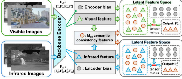
Figure 3. Structure of the Semantic Consistency Inference.
