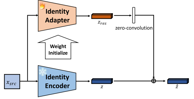
Fig. 8. Identity adapter architecture. A zero-convolution layer is applied to keep the identity encoder's ability at the beginning of training.
