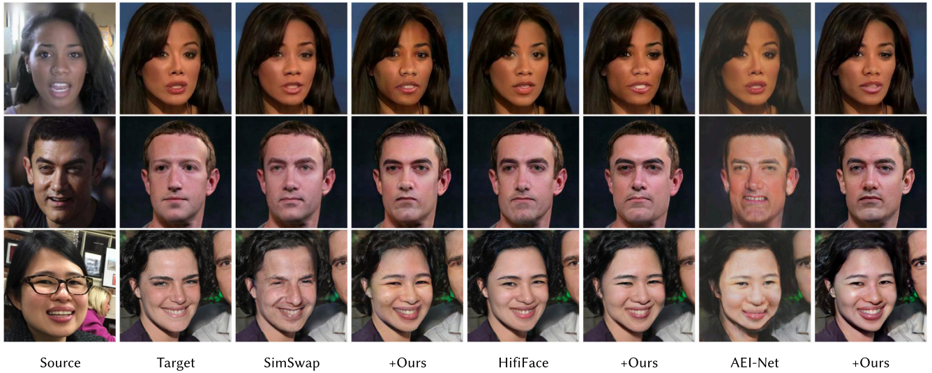
Fig. 13. Qualitative results with different backbones. All of them achieve high ID preserving and the ability to transfer face-shape than base model results.
