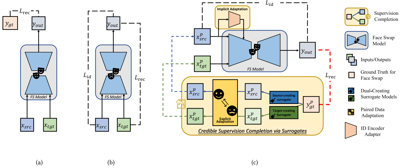
Fig. 6. Comparison between different swapping training frameworks. (a) Face-swapping training with ground-truth swapped image y_{gt} ; (b) current swapping training with ID loss and reconstruction loss; and (c) our CSCS synthesis proxy paired data by dual-creating surrogates from one real image, and adaptation is operated to get the required training data. Credible supervision is applied by L_{rec} between y_{out} and y_{gt} where a real image is utilized to guide swapping. The reserve design of dual surrogates prevents error accumulation from the multi-step synthesis process.
