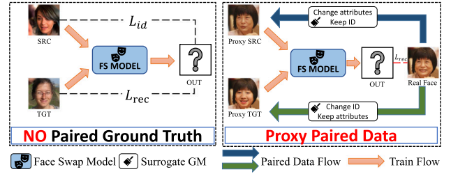
Fig. 2. Overviews of the Credible Supervision Completion via Surrogates framework. Left: The current face-swapping framework, where no ground-truth paired data are used for training and substituted by weakly ID loss and reconstruction loss. Right: The proposed framework, where dual-creating surrogates are applied to synthesize proxy-paired data to train the face swapping.
