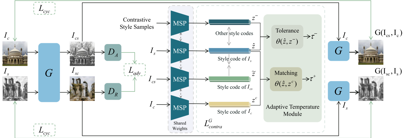
Fig. 3. UCAST consists of a generator G , a parallel contrastive learning scheme relying on a MSP module, and a DE module. The generator is given the content image I_c and the style image I_s and generates images I_{cs} and I_{sc} . Then, I_{cs} and I_s are fed into the MSP module to generate the corresponding style code \hat{z} and \tilde{z} , which are used as positive samples in the style contrastive learning process. The style codes z^- of other artistic images in the style bank are used as negative samples. I_c is fed into the MSP module to generate the corresponding style code z^c . We design an adaptive temperature module that computes the temperature \tau^+ of the positive sample and the temperature \tau^- of the negative samples on the style codes. The contrastive style loss \mathcal{L}_{contra}^G is computed on the temperatures and the style codes. The DE module is based on the adversarial loss \mathcal{L}_{adv} and the cycle consistency loss \mathcal{L}_{cyc} . Style image credit: Giovanni Battista Piranesi/AIC (CC0) [Art Institute of Chicago 2023].
