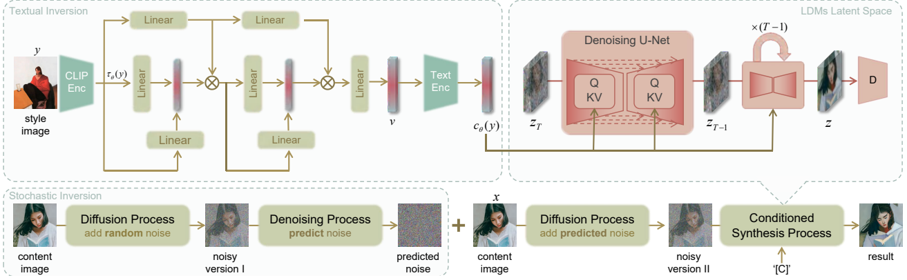
Figure 3. Overview of our InST. We apply the Stable Diffusion Models (SDMs) [42, 50] as the generative backbone and propose an attention-based textual inversion module. During image synthesis, the inversion module takes the CLIP [39] image embedding \tau_\theta(y) of an artistic image y , and gives learned corresponding text embedding v , which is then encoded into the standard form of SDMs’s caption conditioning c_\theta(y) . Through these, the SDMs can generate new images with encoded latent or random noise z_T conditioned on c_\theta(y) .
