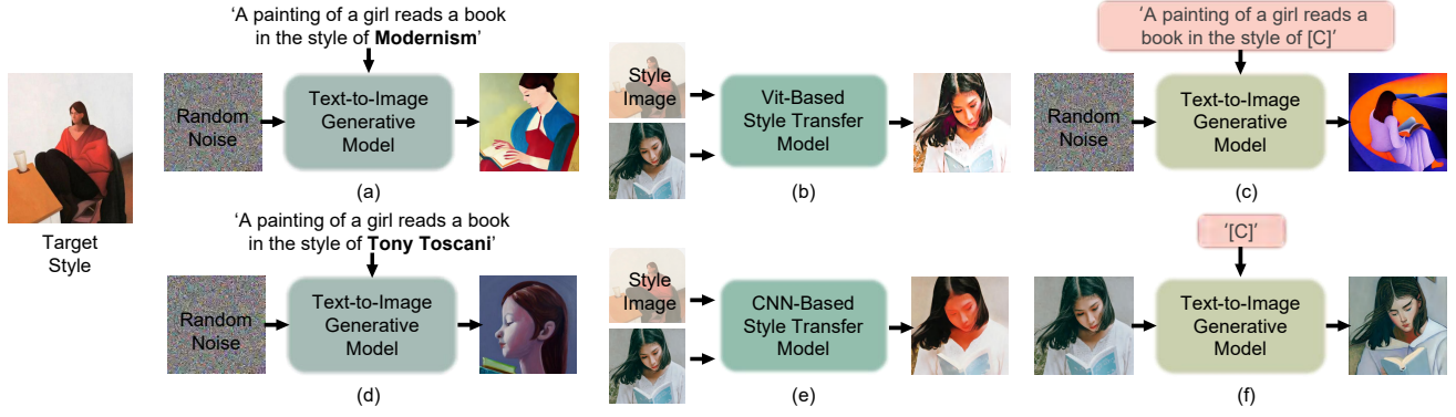
Figure 2. Concept differences between text-to-image synthesis [50], classical style transfer [7, 59] and our InST.
