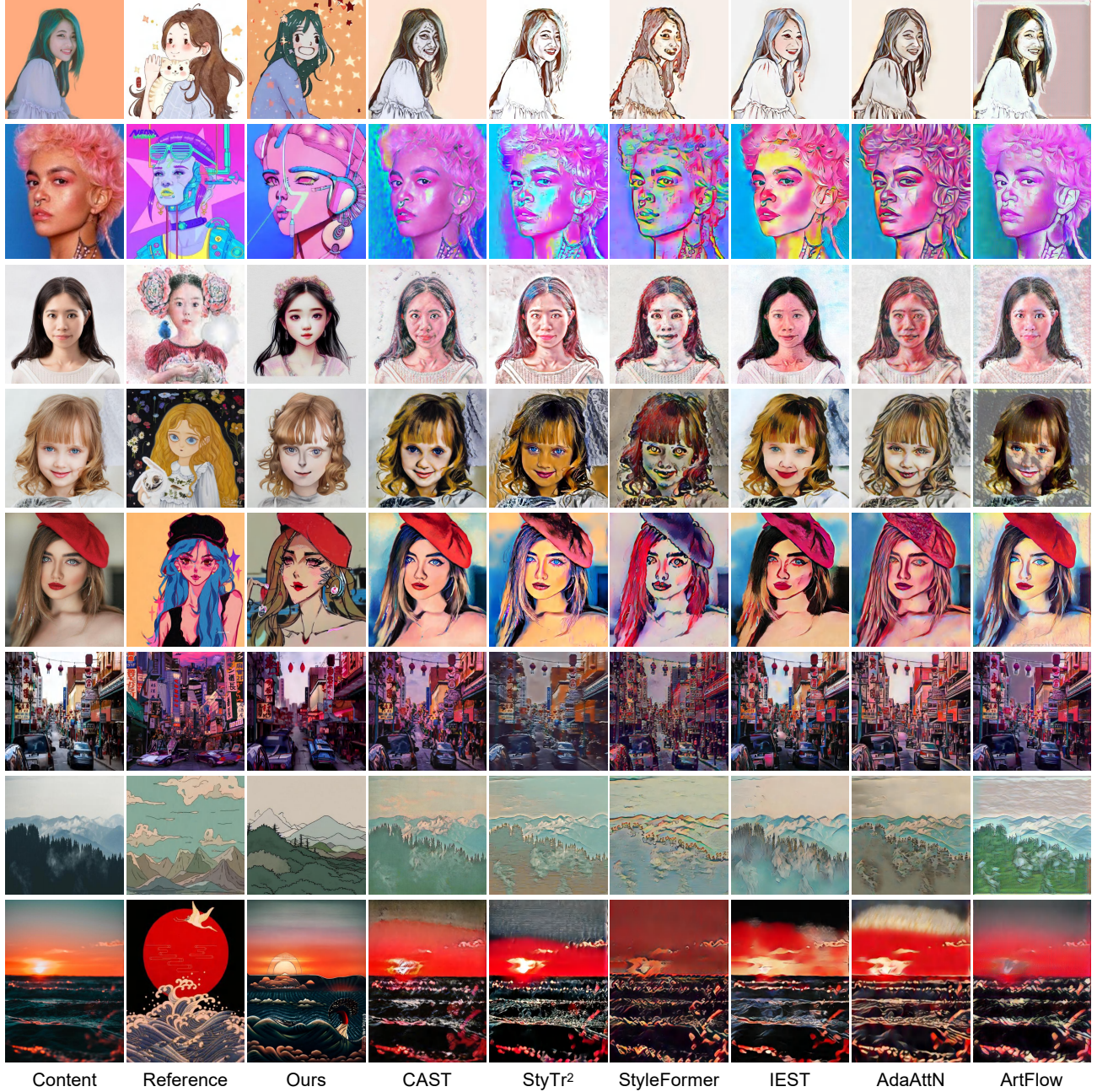
Figure 4. Qualitative comparison with several state-of-the-art image style transfer methods.
