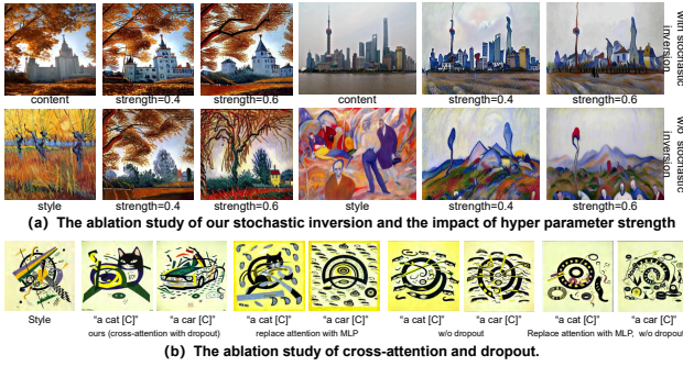
Figure 8. (a) Results of the ablation study on our stochastic inversion, hyper-parameter Strength , (b) attention module and dropout.
