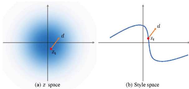
Fig. 5 Style fine-tuning in z space and style space. Manipulation in style space leads to an out-of-manifold result.
