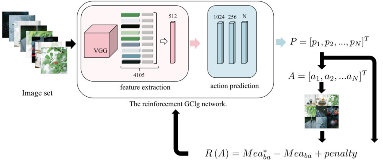
Fig. 6. Structure of the reinforcement GClg generation network. The network takes all the images as input and will output an action probability distribution P according to the image features and the current image arrangement order. An image exchange action will be taken according to multinomial distribution sampling based on P . The reward will be calculated by the variance between the balance measurement before action taken ( Mea_{ba}^* ) and balance measurement after action taken ( Mea_{ba} ). A penalty item is also added to the reward function for an effective and fast search. Then, the images in new arrangement order will be sent to the network again until the terminal action or the max step.
