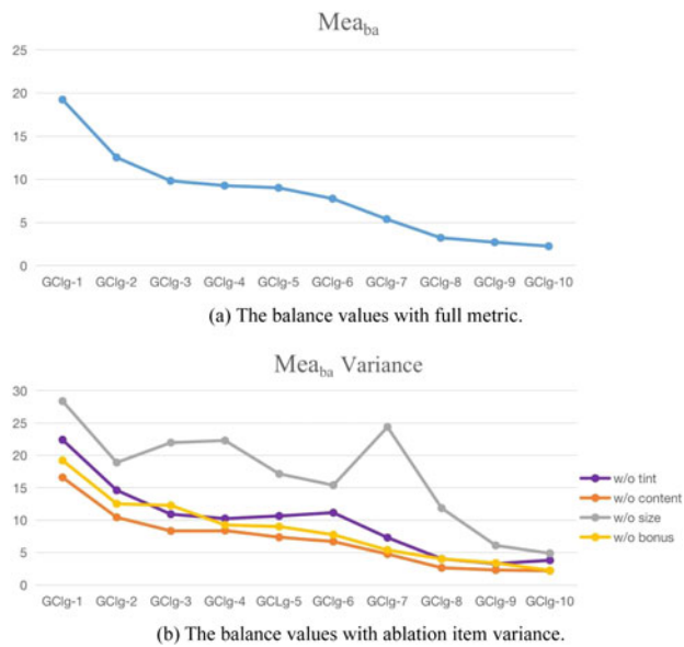
Fig. 10. Illustration of balance value variance in Fig. 9.
