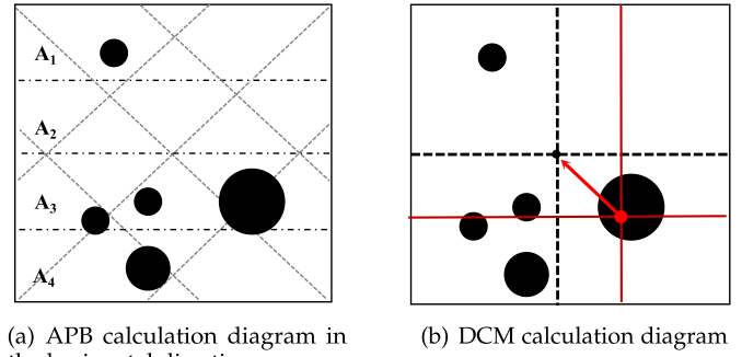
Fig. 4. Basic visual balance calculation diagram.
