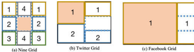
Fig. 7. Three typical GClg templates.
