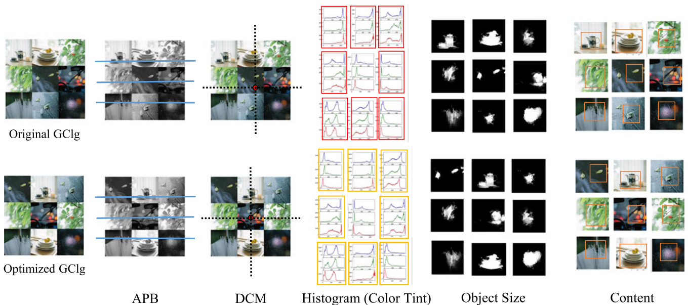
Fig. 11. Measured item visualization of different collages. The yellow box in the content column marks the main content in the image. Please zoom in the document to see the details of the diagrams.
