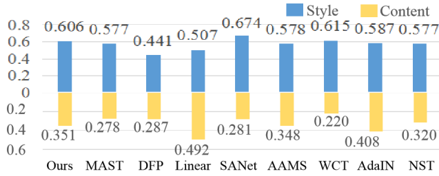
Figure 6: Classification accuracy.
