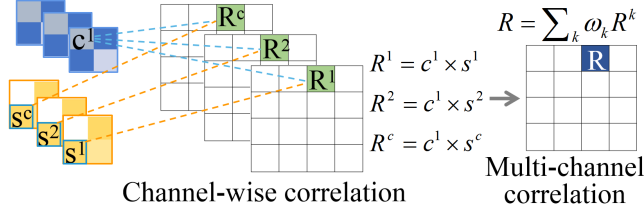
Figure 3: Correlation matrix CO. R is the element of CO.
