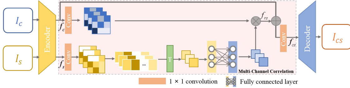
Figure 2: Overall structure of MCCNet. The green block represents the operation of the feature vector multiplied by the transpose of the vector. \otimes and \oplus represent the matrix multiplication and addition. I_c , I_s and I_{cs} refer to the content, style and generated images, respectively.
