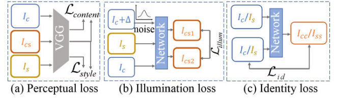
Figure 4: Loss function.
