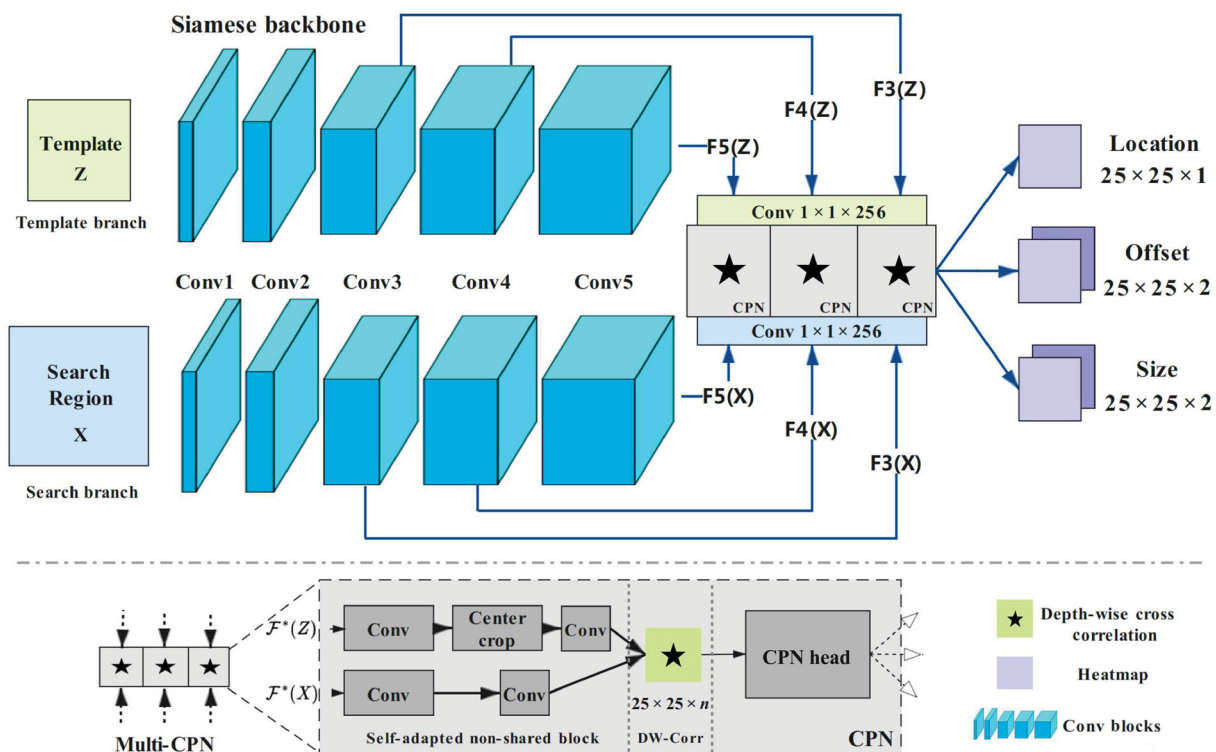
Fig. 1 SiamCPN. Above: the entire framework. Blue boxes: conv-blocks in ResNet-50. The output of Conv3, Conv4, and Conv5 are fed into CPN. Gray block: CPN module. ★ denotes depth-wise cross-correlation. Our network produces three 25 \times 25 outputs. Below: architecture of the CPN module. Before input to the CPN, channels are reduced to the same size. The self-adapted block forms the first part of the CPN module. Only the structure of a single output branch is shown.
