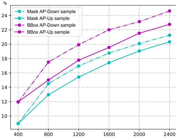
Fig. 1. Comparisons of different input sizes on the MVD detection benchmark. Training samples are obtained by downsampling the original high-resolution images to different scales or upsampling from half-sized images.
