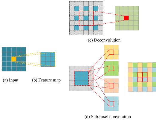
Fig. 3. Comparison between how deconvolution and sub-pixel convolution layers conduct the upsampling progress. (a) Input pixels. (b) Output feature map after 3 \times 3 convolution. (c) Deconvolution and (d) sub-pixel convolution are two different feature upsampling ways. The deconvolution layer first pads zeros and then conducts a standard 3 \times 3 convolution, whereas the sub-pixel embeds information to channels using a 3 \times 3 \times 4 kernel and then rearranges it periodically.
