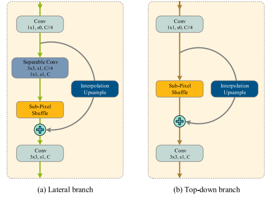
Fig. 4. Residualized sub-pixel convolution block. The two blocks are applied at upsampling operations for (a) lateral and (b) top-down connections in our guided feature upsampling module.
