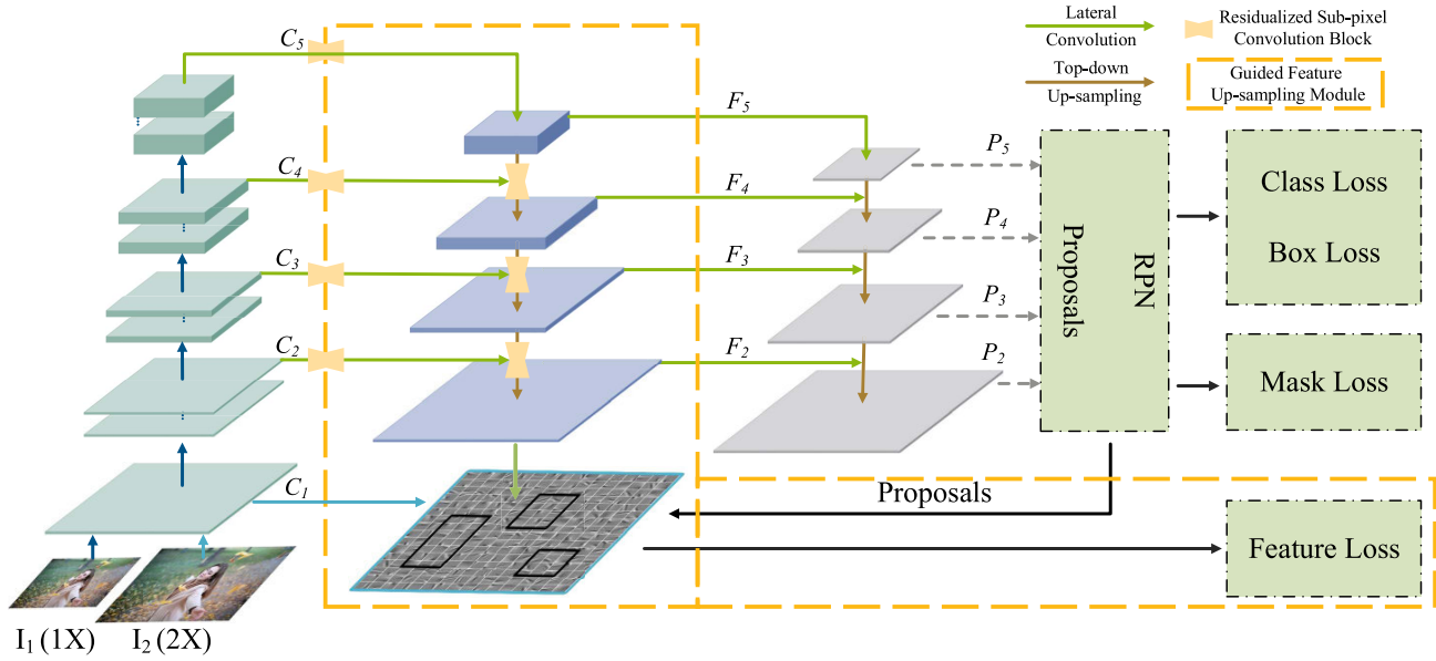
Fig. 2. Overall architecture of our approach. The components in dashed yellow bounding boxes are proposed in this work, whereas the others belong to the FPN-based Mask R-CNN framework. The classification and regression heads of RPN [5] are omitted for clarity. The proposed guided feature upsampling module locates right after the bottom-up pathway of the backbone network and learns the upsampled feature for each stage \{C_2 - C_5\} guided by real larger feature C_1 . The learned features \{F_2 - F_5\} are fed to the second top-down pathway and finally accessed to the detection block.
