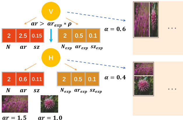
Fig. 4. Illustration of the coarse adjustment of one node. Given that the condition (ar > ar_{exp} \cdot \rho) is met, we change the division type from Vertical to Horizontal and adjust \alpha according to Equation. (15) The node area is accordingly adjusted when the entire tree updates.
