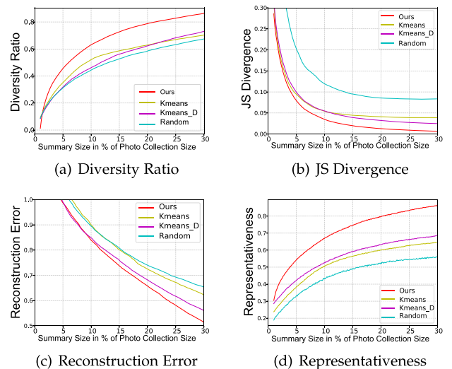
Fig. 6. Quantitative comparison results of our summarization method and the three baseline methods by using the four metrics.
