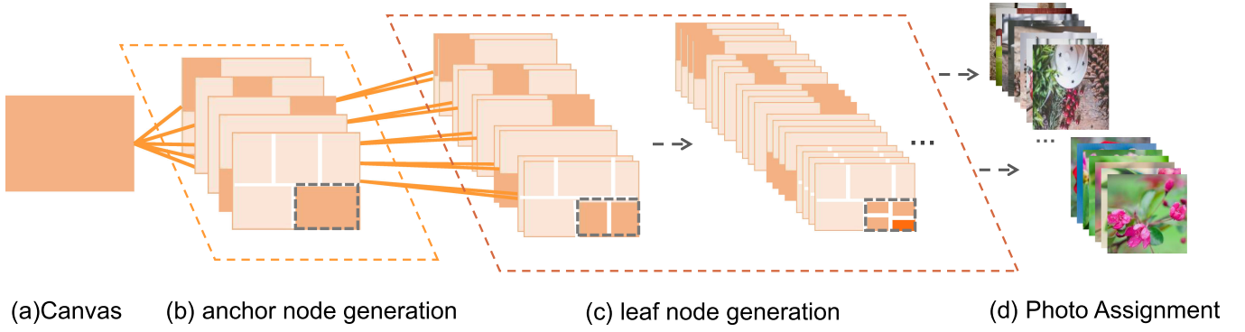
Fig. 3. Illustration of our layout initialization method. The root node (a) is divided into |S_a| anchors nodes based on the anchor images in the first stage (b) of tree construction. In the second stage (c), each anchor node is recursively split by binary partition until (d) each leaf node is only associated with one image.
